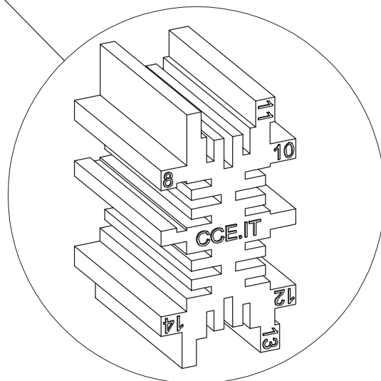
UNIVERSAL CENTERING JIG (for glasses from 8 mm up to 14 mm thick)
